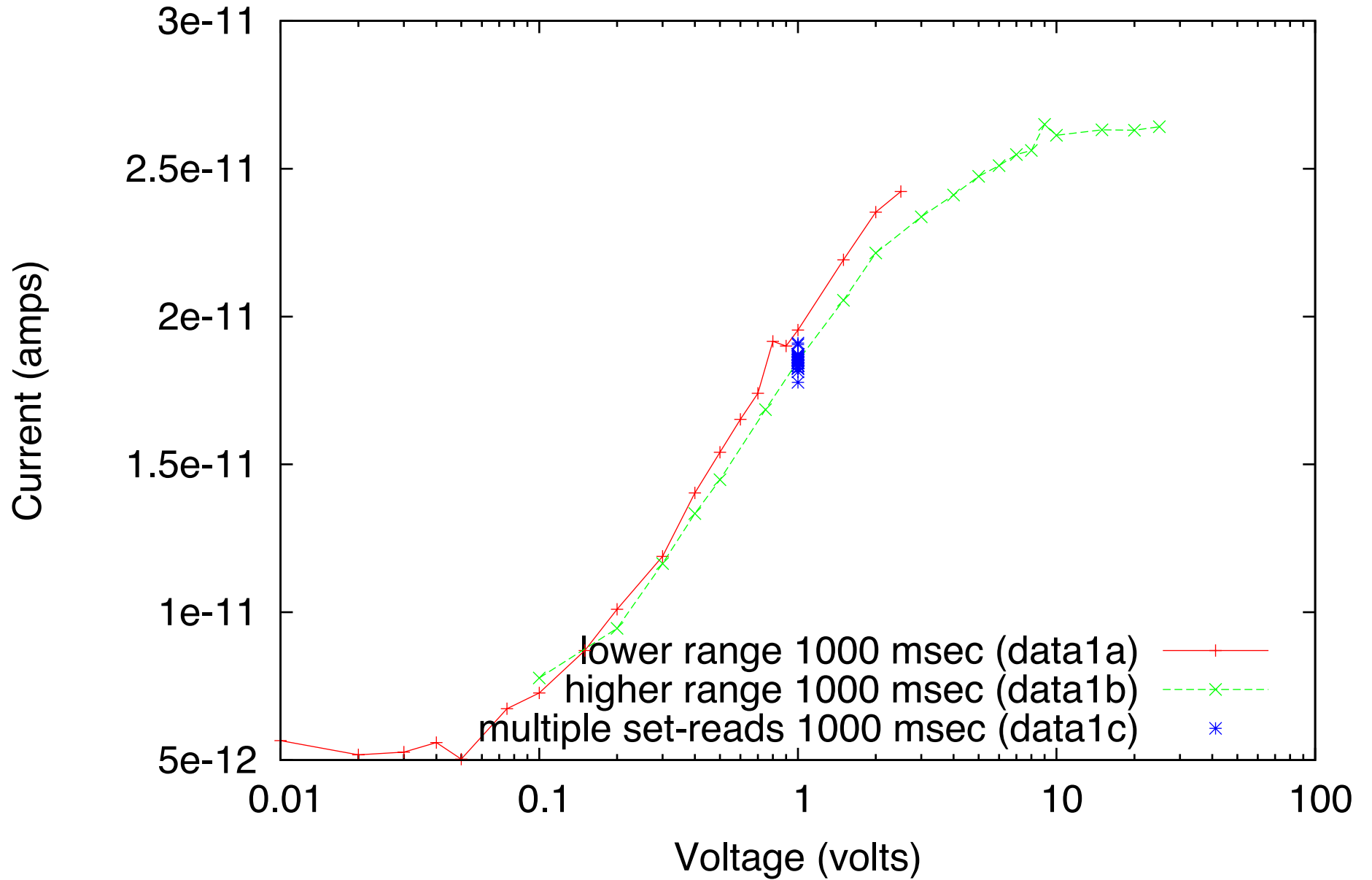
Tube 2 IV measurements demo
