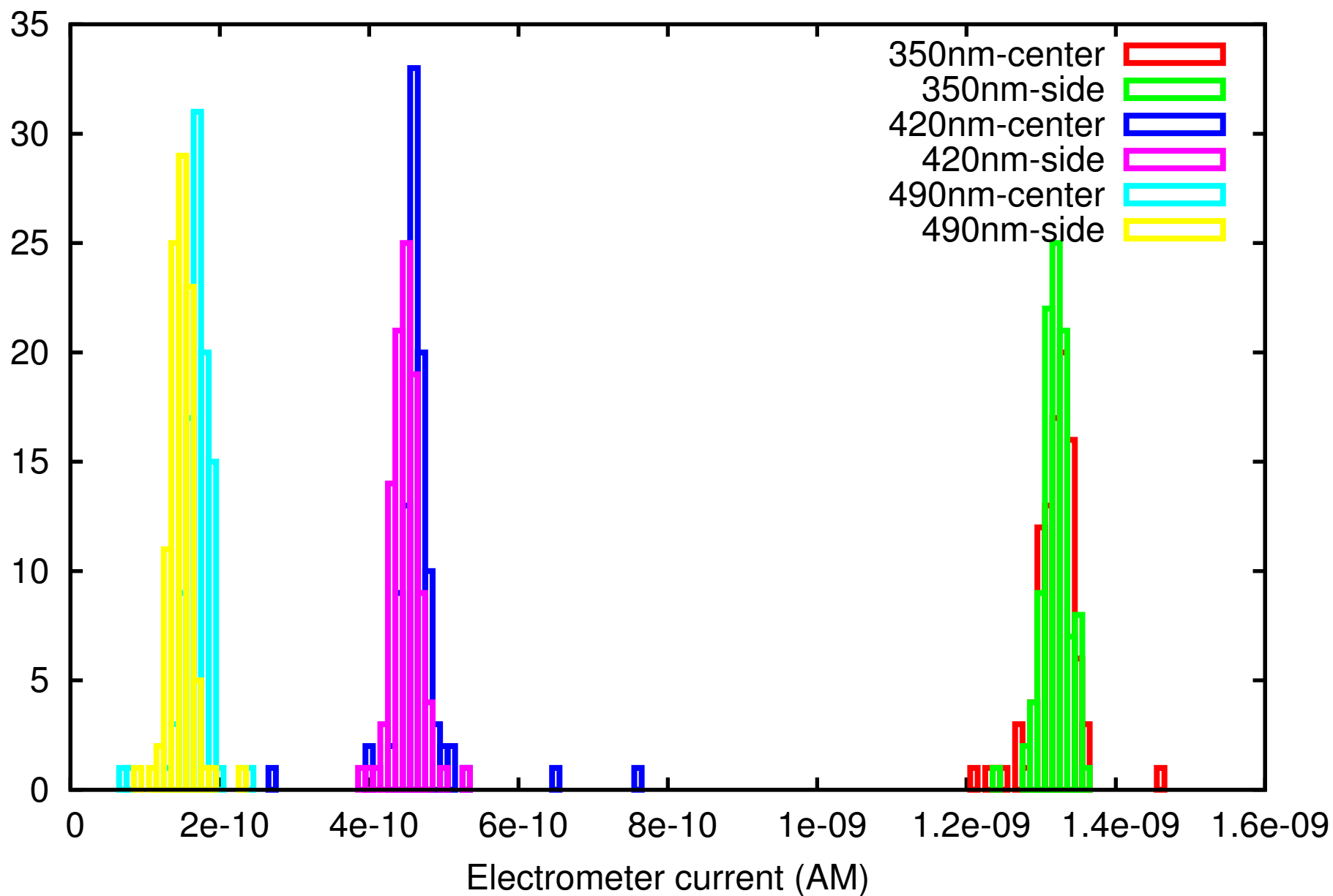
Histogram Raw Data from QE Mapping at 350,420 and 490 nm : Current(A)
