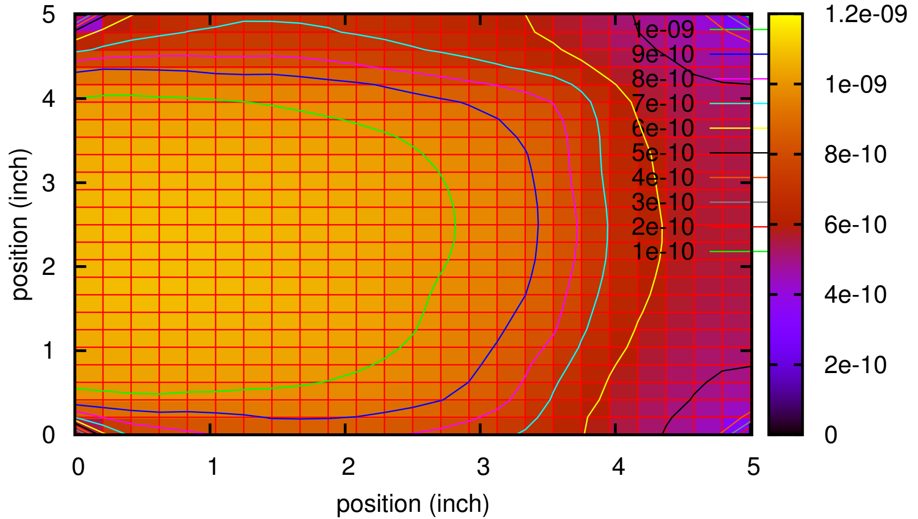
Raw Data QE Mapping at 350nm: X Y Current(A)
