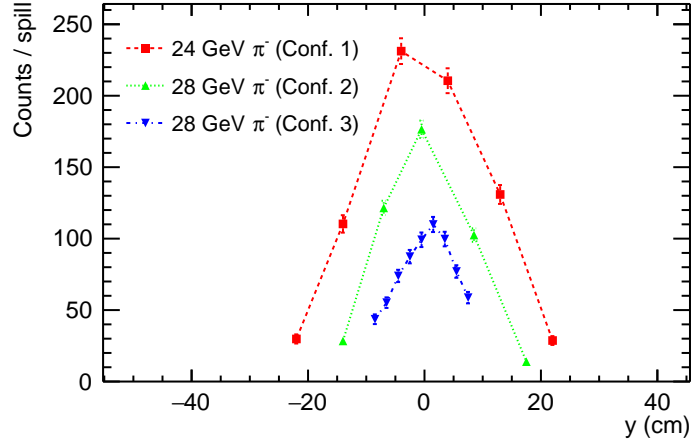
Figure 4: Muon beam profile scan in the vertical direction for several different pion beam energies and various configurations of the counters described in Table 1. The reference point for the y -coordinate is the beam center, located at 156 cm from the floor.
